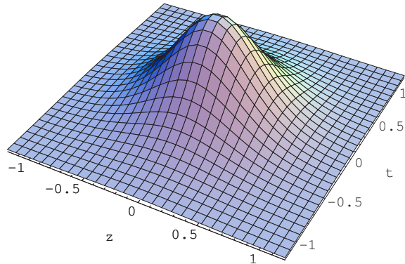
Figure 2: Action density of the YM instanton as function of z , t at fixed x = y = 0 .
